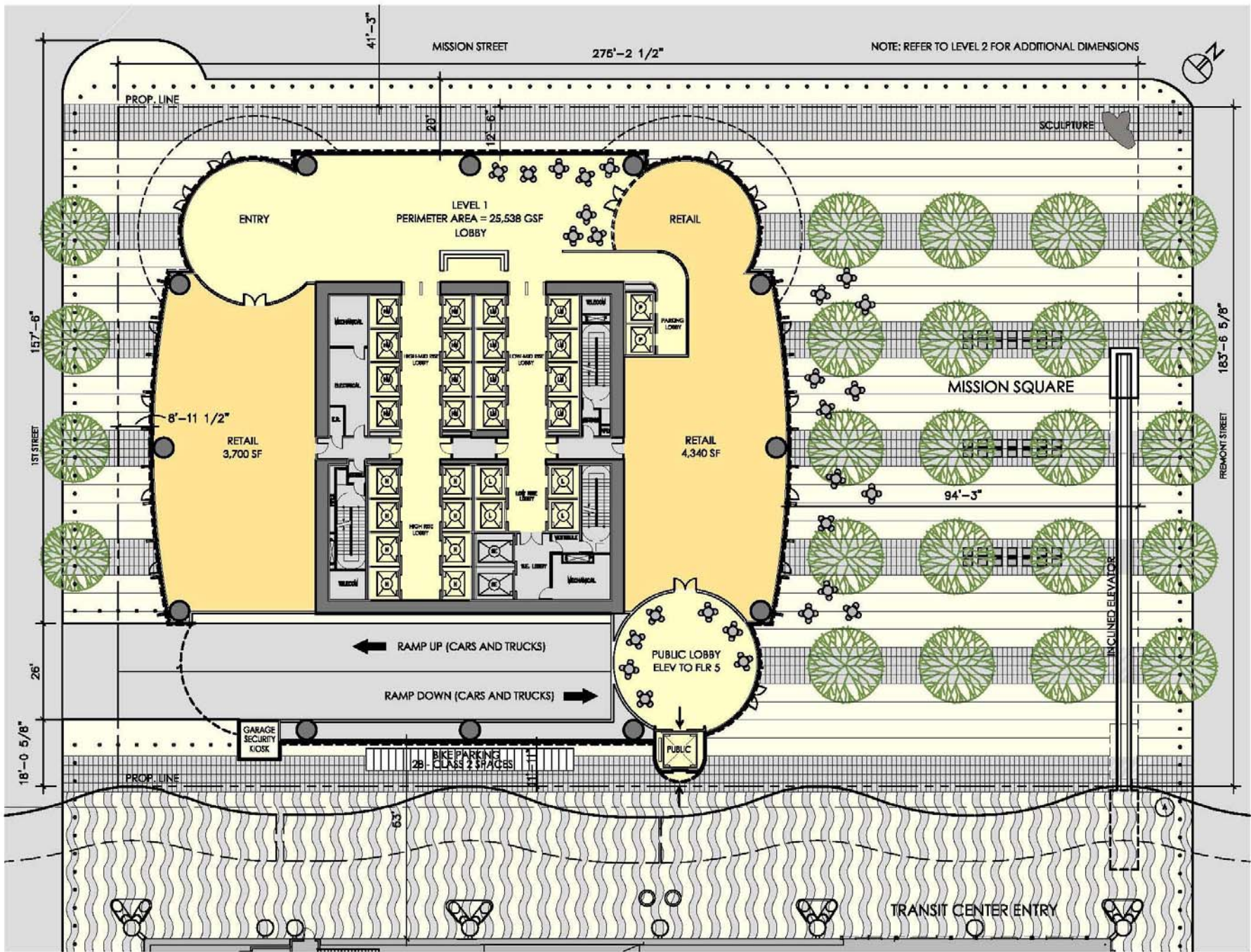
TOWER - GROUND FLOOR
