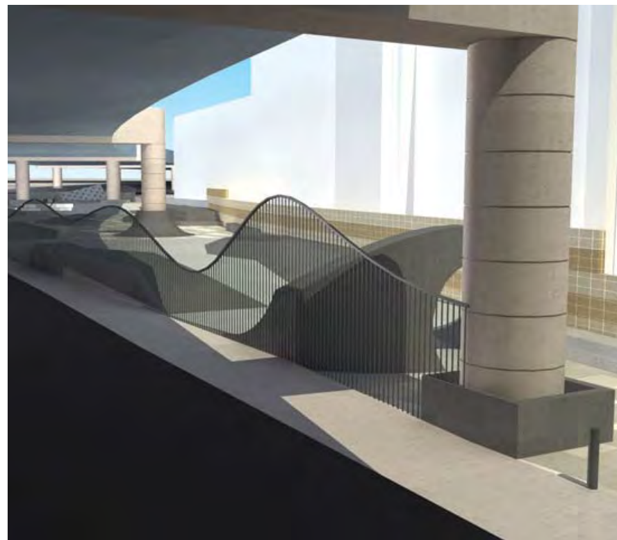
SOMA Skatepark, San Francisco CA (construction planned 2013)
